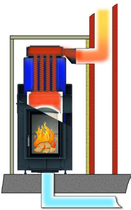
Boiler operation with direct connection
