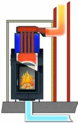
Boiler operation with direct connection
