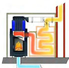
Heat storage mode with Moritz's flap
