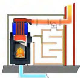
Boiler operation with Moritz's flap
