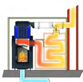
Heat storage mode with Moritz's flap
